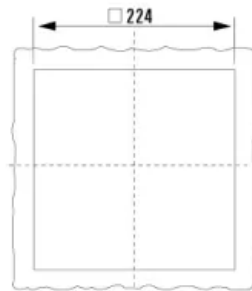
Cut-Out Dimensions
