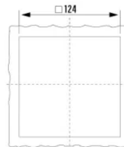
Cut-Out Dimensions
