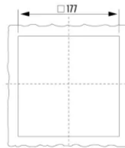
Cut-Out Dimensions
