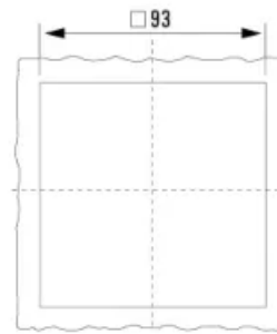
Cut-Out Dimensions
