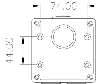
MOUNTING HOLE DETAIL
